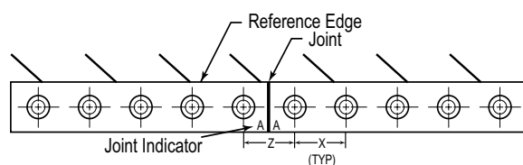
Figure 6. Butt jointed rails
